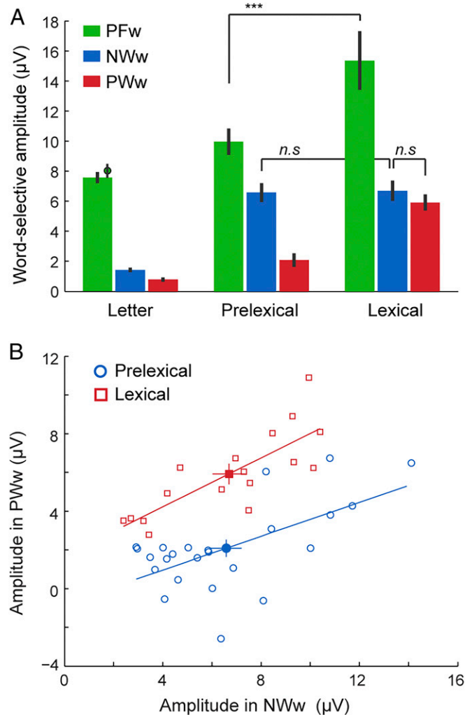
Fig. 8. Amplitude quantification across conditions and processing levels. (A) Response amplitudes were quantified as the average of the amplitudes across recording contacts, separately for each processing level (letter, prelexical, and lexical) and each condition (PFW, NWW, and PWW). The additional data point over the left-most column represents the averaged response amplitude over contacts located in the same anatomical regions as the prelexical and lexical contacts (latFG, medFG, antFG, antOTS, and ant-CoS). (B) Relationship between the amplitude in the PWW and the NWW conditions, separately for the prelexical and the lexical recording contacts. Each white-filled point is a single contact, and the mean across contacts is shown as filled markers. Lines represent the least-square linear fit computed separately for prelexical and lexical contacts. Error bars are the SEM.
